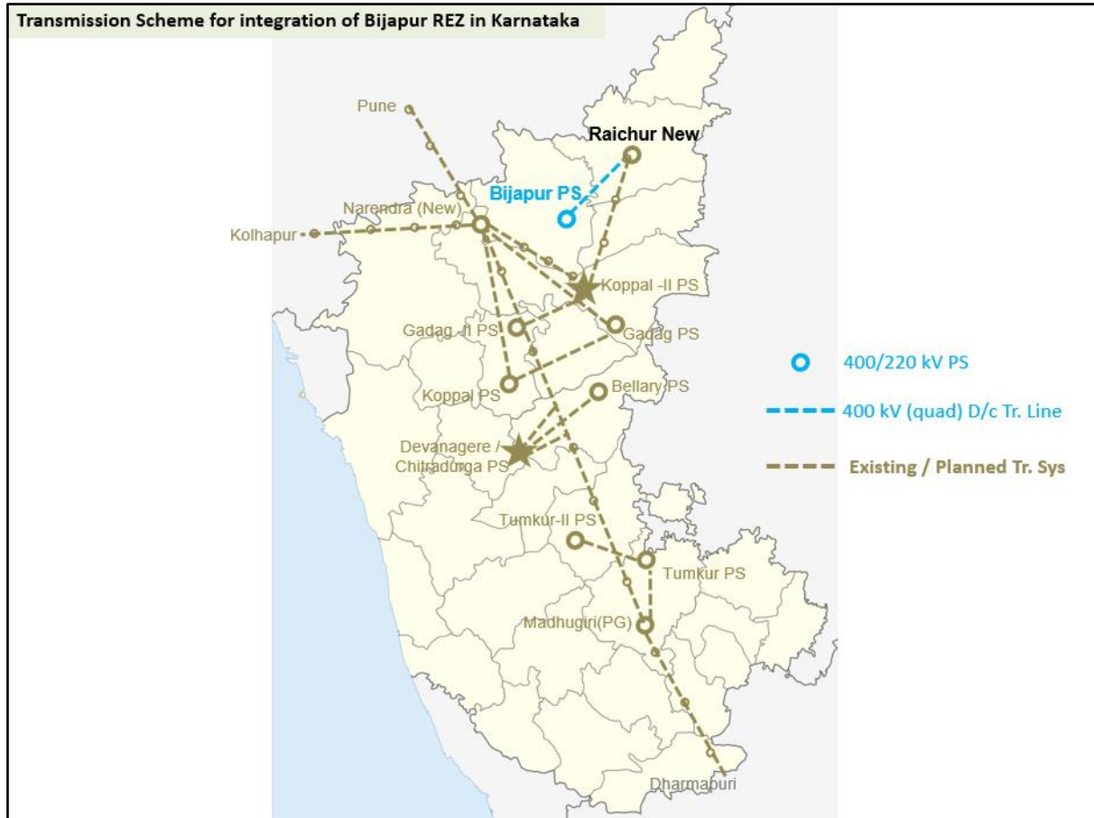
Fig-1 : Transmission Scheme for integration of Bijapur REZ in Karnataka
